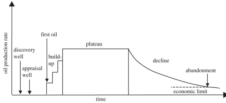
Figure A3: Standard Offshore Oil Production Curve
