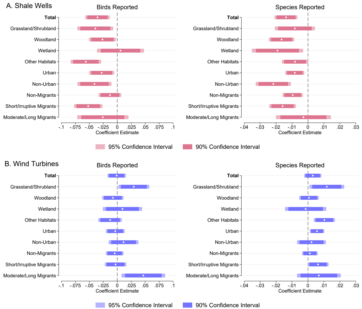
Figure A11: Correlated Spatial Random Effects Model
