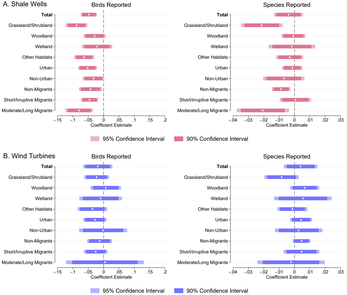
Figure A10: Poisson Model with Random Effects and Grid-Square Clustered Errors
