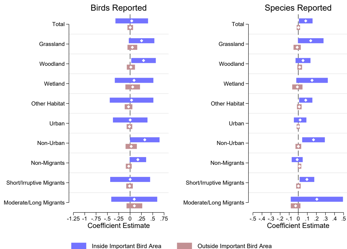
Figure A18: Effects of Wind Turbine Arrival Inside/Outside Important Bird Areas (Disaggregated by Characteristic)
