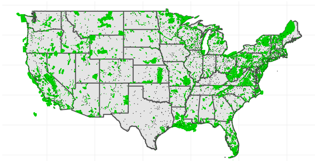
Figure A17: CBC Circle Locations Relative to Important Bird Areas (in Green)
